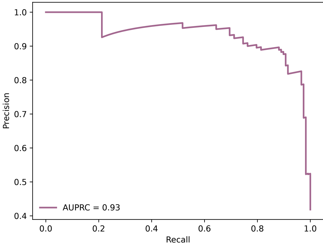
LOGISTIC Precision-Recall Curve
